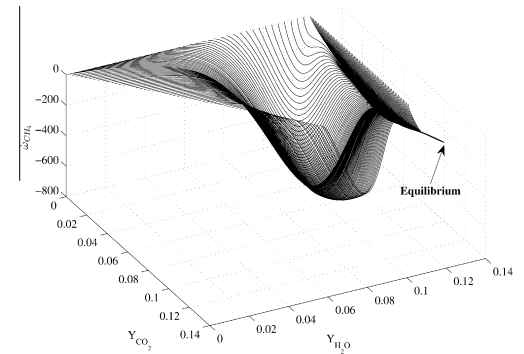
Fig. 1. Illustration of two-dimensional flame-generated manifold (2D-FGM) for methane-air combustion showing the production rate of CH 4 as a function of the progress variables c_1 and c_2 .
