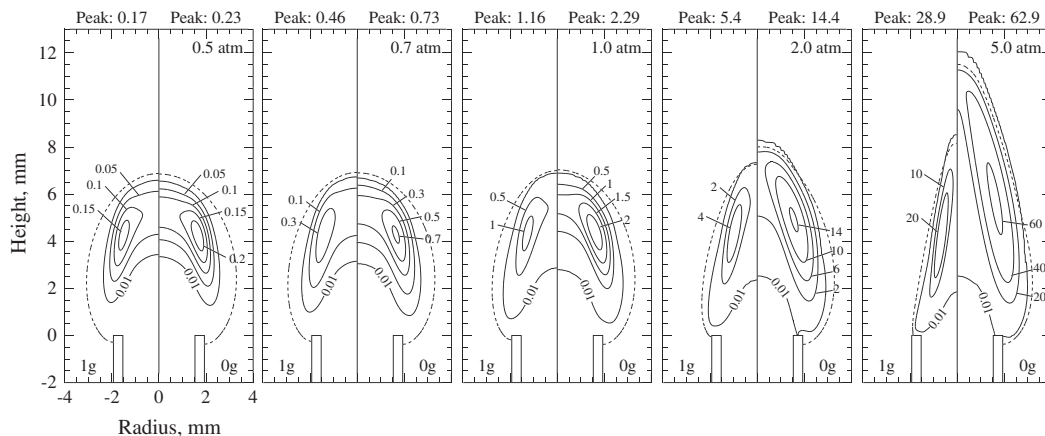
Fig. 6. Predicted contours for soot volume fraction in the normal-gravity (left) and zero-gravity (right) flames. Units in ppm. Dashed black lines denote the location where the mixture fraction is equal to the stoichiometric value. Visible flame shape is denoted by the 0.01 ppm contour.
