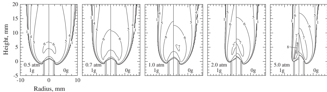
Fig. 11. Predicted contours of the divergence of the radiative heat flux, \nabla \cdot \mathbf{q}_{\text{rad}} . Contours correspond to \log_{10}[\max(-\nabla \cdot \mathbf{q}_{\text{rad}}), 1 \text{ W/m}^3] where the units of \nabla \cdot \mathbf{q}_{\text{rad}} are 1 \text{ W/m}^3 .
